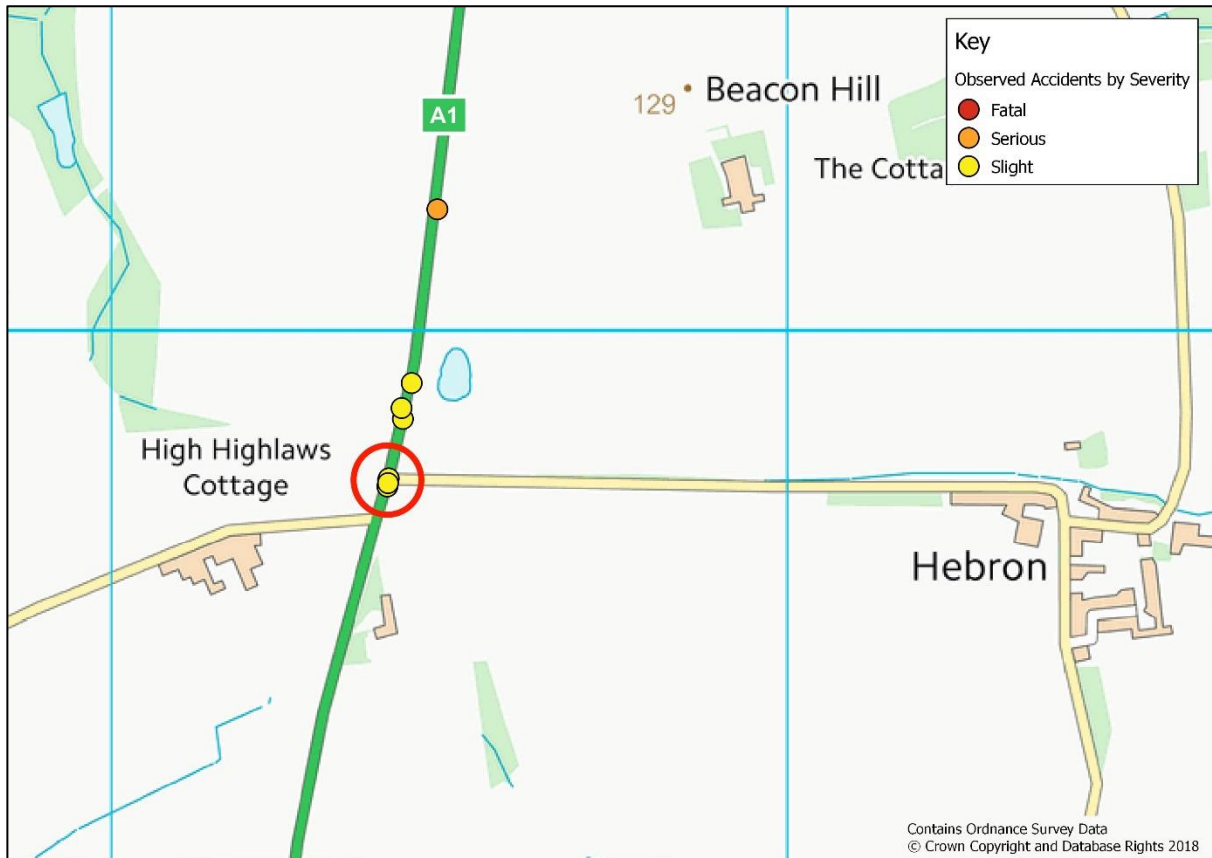
Figure 16: Accident Cluster at Hebron Junction
