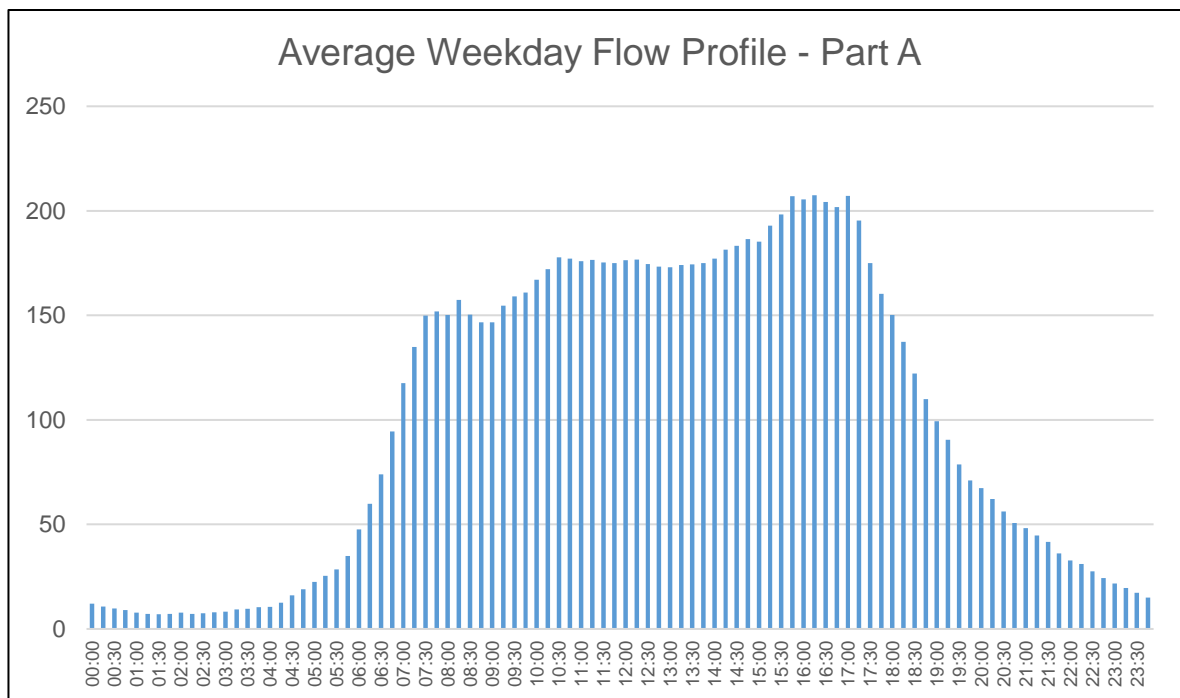
Figure 8: Average 2017 Weekday Two-Way Flow Profile (WebTRIS Counts) – Part A
