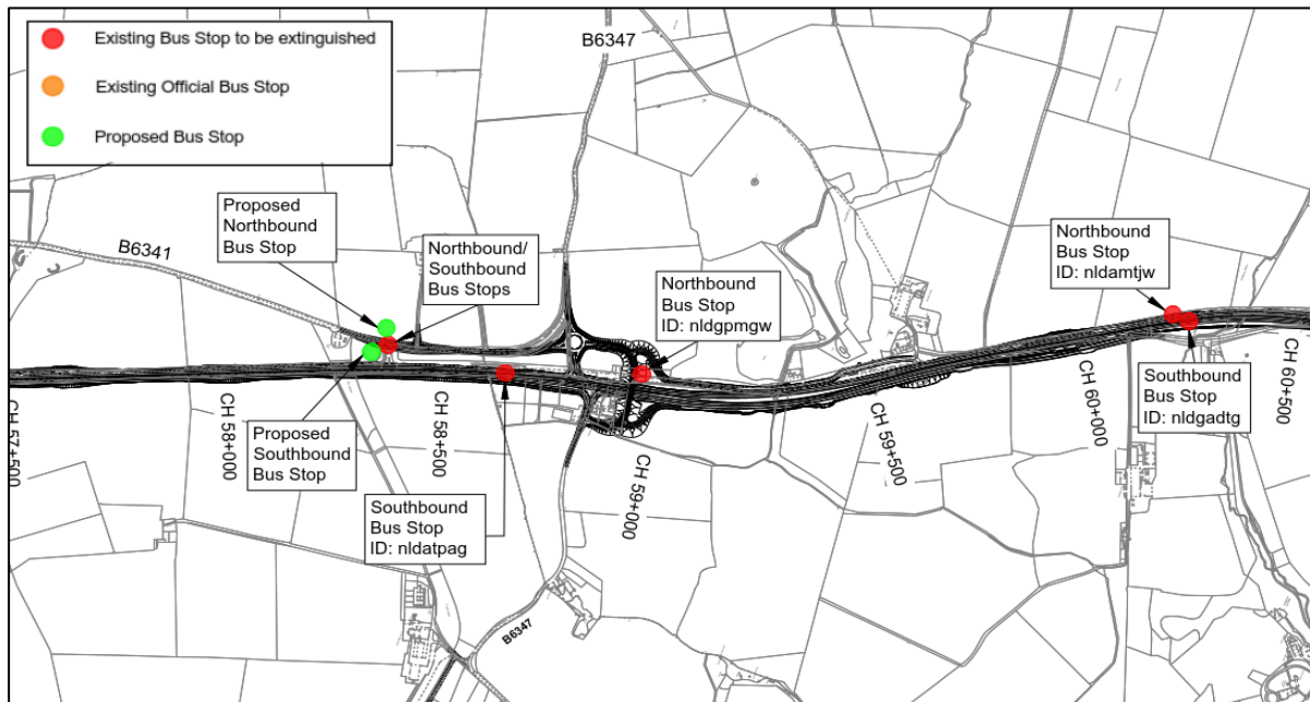
Figure 25: Existing and Proposed Bus Stops – Part B
